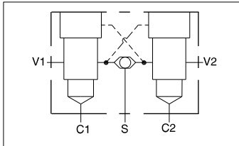
Two cavity 90 degree cross-piloted body with shuttle for load control applications.
