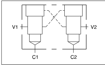
Two cavity 90 degree cross-piloted body for load control applications.
