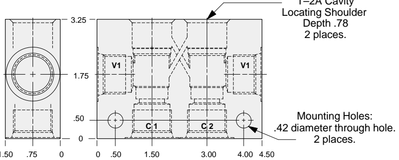
Two cavity 90 degree cross-piloted body for load control applications.
