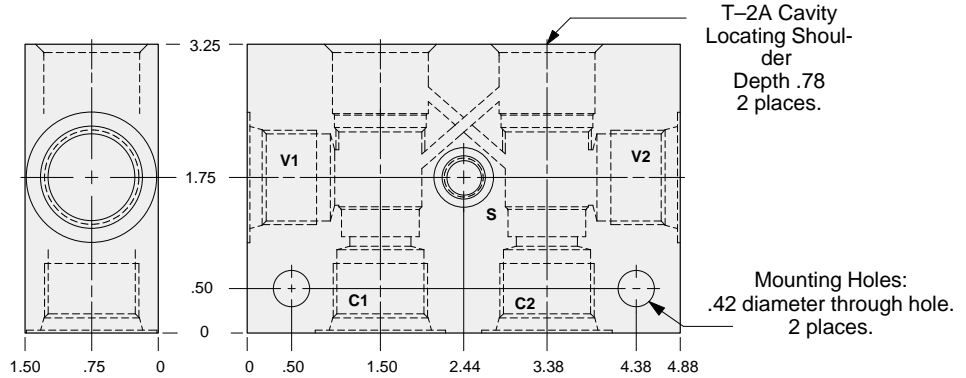
Two cavity 90 degree cross-piloted body with shuttle for load control applications.
